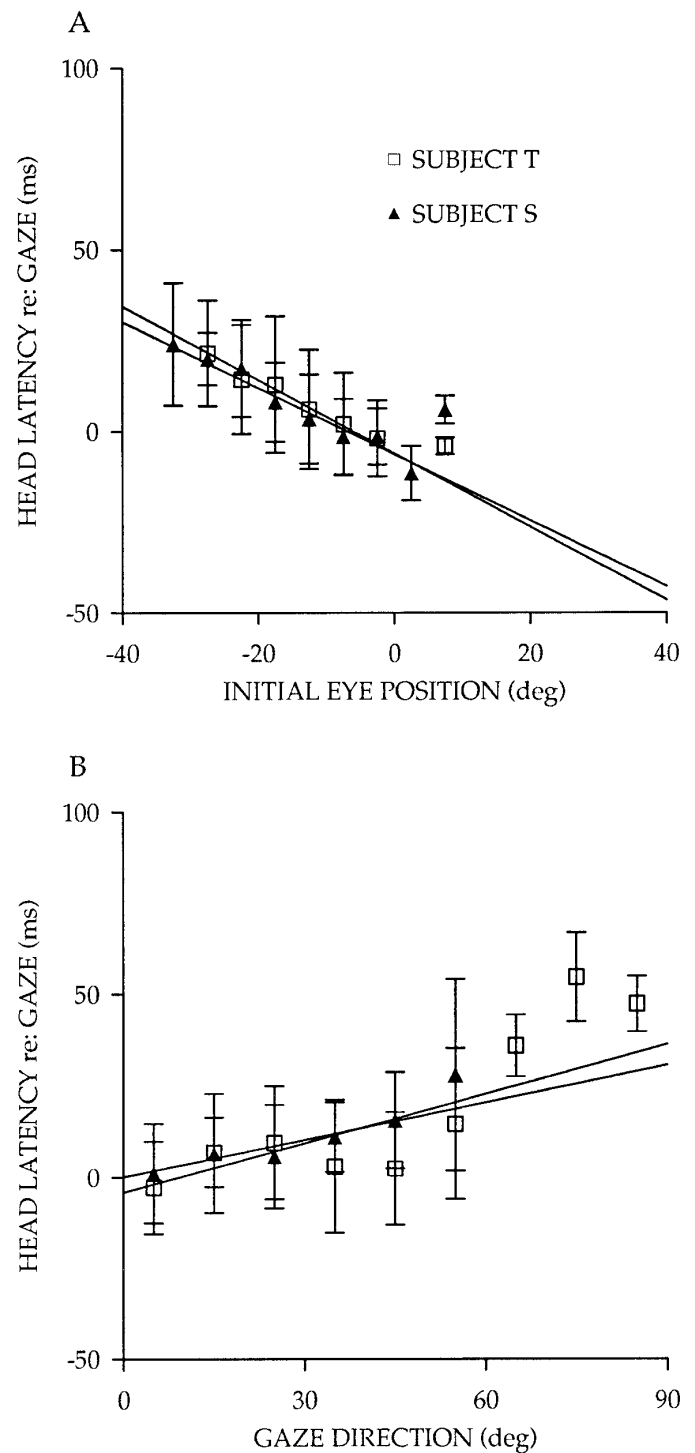
FIG. 19. A: effect of initial eye position on the relative timing of eye and head movements for monkey T ( \square ) and monkey S ( \blacktriangle ) for constant-amplitude gaze shifts ( 60\text{--}65^\circ ). Binwidth for calculating means \pm SD was 5^\circ , and data are fit with a least-squares regression line. Monkey T : n = 218 , r = -0.45 , sl = -1.0 . Monkey S : n = 122 , r = -0.47 , sl = -0.94 . B: effects of movement direction on the latency of head movements relative to gaze onset for gaze shifts between 60 and 65^\circ . Binwidth for calculating means \pm SD was 10^\circ . Monkey T : n = 219 , r = 0.58 , sl = 0.45 . Monkey S : n = 201 , r = 0.45 , sl = 0.34 . Negative initial eye positions are contralateral to movement direction. Negative head latencies relative to gaze onset: head movement onset preceded gaze onset. Gaze directions are relative to the horizontal meridian and include movements with both upward and downward vertical components.
