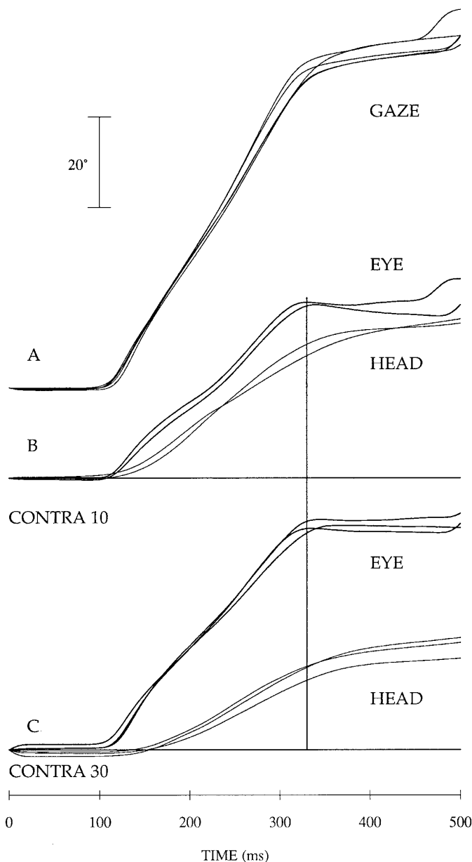
FIG. 13. A: horizontal gaze position for 5 individual movements directed along the horizontal meridian. Gaze amplitude = 68–72°. B: eye and head position traces for 2 of the 5 movements in A initiated when the eyes were deviated in the orbits by 10° contralateral to the direction of movement. C: eye and head position traces for the remaining 3 trials initiated when the eyes were 30° contralateral in the orbits. Scale bar in A applies to A–C.
