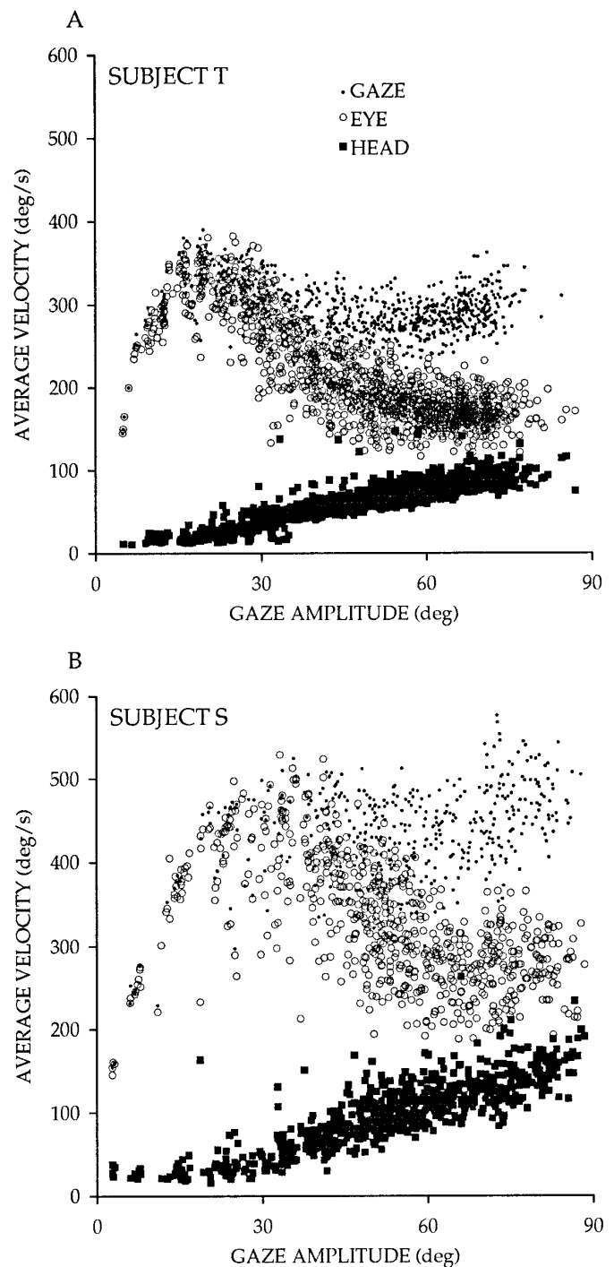
FIG. 9. Comparison of average gaze ( \bullet ), eye ( \circ ), and head ( \blacksquare ) velocities during gaze shifts ranging in amplitude from \sim 5 to 90^\circ directed along the horizontal meridian ( \pm 10^\circ ), initiated with the eyes centered ( \pm 10^\circ ). A: data from monkey T ( n = 318 ). B: data from monkey S ( n = 272 ).
