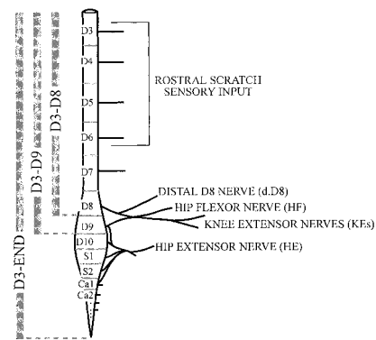
FIG. 1. Diagram of the turtle spinal cord, indicating sensory and motor components of the rostral scratch reflex (right) and the spinal segments included in D_3 -end, D_3 - D_9 and D_3 - D_8 preparations (left). All preparations had a complete spinal transection just posterior to the forelimb enlargement between segments D_2 and D_3 . D_3 -end preparations had intact spinal cords posterior to the D_2 - D_3 transection site. D_3 - D_9 and D_3 - D_8 preparations had a 2nd transection between segments D_9 - D_{10} or D_8 - D_9 , respectively. Fictive rostral scratch motor patterns were elicited by electrical or mechanical stimulation of the shell in the right and/or left rostral scratch receptive field(s) and recorded bilaterally from hindlimb muscle nerves (shown on the right side only). Electroneurographic (ENG) recordings were obtained from a knee extensor (KE) nerve (either AM-KE or FT-KE), a hip flexor (HF) nerve (VP-HP), and either a hip extensor (HE) nerve (HR-KF) or the distal D8 nerve (d.D8), which exhibits HF- and HE-correlated motor bursts. See METHODS for a more detailed identification of peripheral nerves and a description of surgical procedures.
