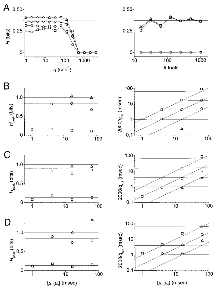
FIG. A1. Metric-space results for simulated data. Test of the suitability of the metric-space method for estimating information and temporal precision when the number of spikes per trial is low. A: bias-corrected information as a function of the cost q (left) and the number of simulated trials (right). Left: different curves represent different numbers of simulated trials: 16 (open squares), 64 (open circles), 128 (open triangles), and 1,024 (inverted open triangles). Right: different curves represent different values of q : 1 (open squares), 8 (open circles), 64 (open triangles), and 512 (inverted open triangles) s^{-1} . B–D: peak information ( H_{\text{peak}} ) and temporal precision limits ( 2,000/q_{\text{cut}} ) derived from fits to the information curves. Left: solid lines show expected information values from a likelihood-ratio analysis. Right: solid lines show expected temporal precisions for different mean separations (slanted lines) and standard deviations (horizontal lines) of the Gaussian distributions that are used to generate spike times. Symbols correspond to different ratios of mean separation to standard deviation: 1 (open squares), 4 (open circles), and 16 (open triangles). B: 1 spike/trial. C: 2 spikes/trial; spike-time distributions within a trial have a mean separation of 32 ms. D: 2 spikes/trial (same data as in C) but only the 1st spike in each trial is analyzed.
