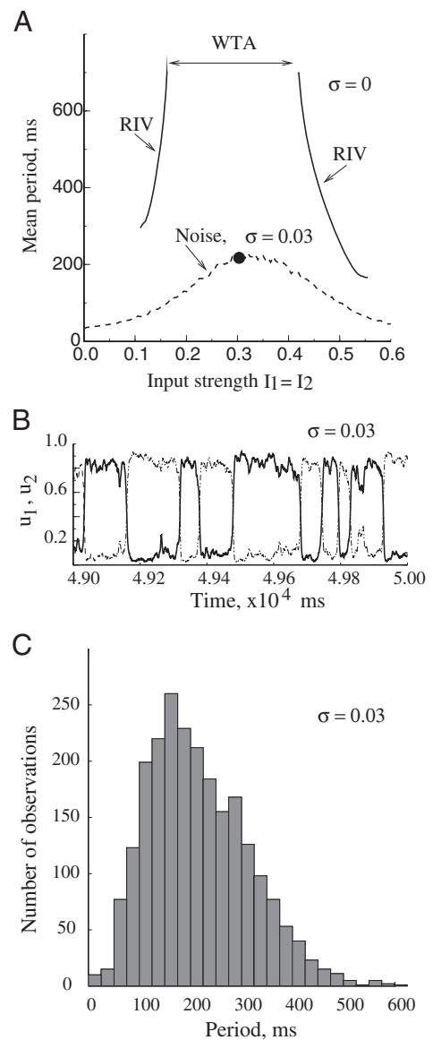
FIG. 6. A: period T of network oscillation vs. input strength for the depression-LC model in the absence (solid line, identical to the one in Fig. 4A) and in the presence (dashed lines) of noise with \sigma = 0.03 . Inhibition strength parameter is \beta = 0.6 . For values of the other parameters, see METHODS. B: typical time course of the network activity, calculated for the input strength value I_1 = I_2 = 0.3 (marked by a filled circle in A) and noise strength \sigma = 0.03 . C: distribution of the periods durations for this model, calculated for the input strength value I_1 = I_2 = 0.3 and noise strength \sigma = 0.03 . Standard deviation over mean ratio is 0.45.
